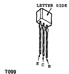
2SA1175-HFE 2SC2785-HFE
