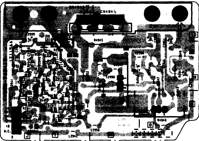
WB [VELOCITY MOD.] (KV-27V36/29V36C/29V76M ONLY)
